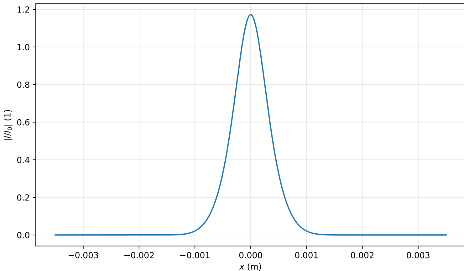
Intensity profile I(x, y = 0, z = 0.637m)/I_0 , P_{in}=0.8P_{cr} , artificial time
